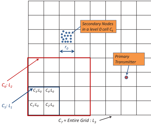
Fig. 1. Cells of different levels in a hierarchy with branching factor b = 4 . C_i : L_j denotes cell C_i at level j .
