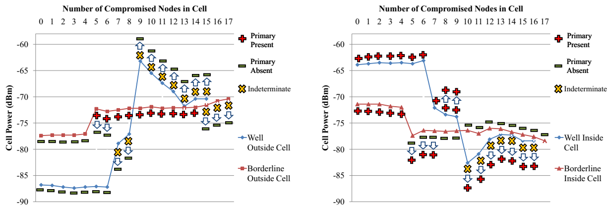
Fig. 6. Exploitation (left) and Vandalism (right) by Average Attackers. Arrows represent change of final detection outcome based on extensions in Section VI.
