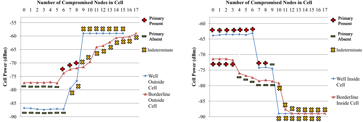
Fig. 2. (left) Exploitation by +15dB Naive Attackers. ML detector is beat when 7 (4) nodes are compromised in the well-outside (borderline-outside) cell. (right) Vandalism by -15dB Naive Attackers. ML detector is beat when 7 (3) nodes are compromised in the well-inside (borderline-inside) cell.
