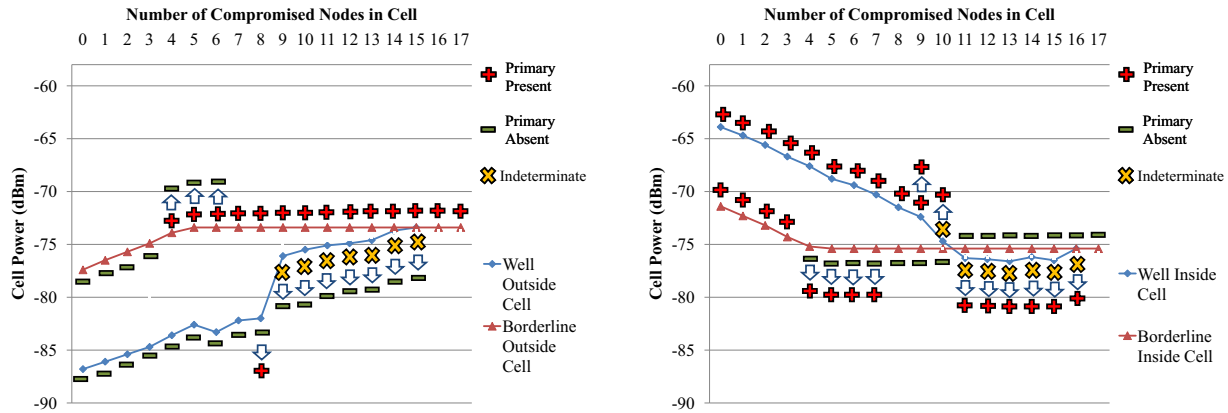
Fig. 7. Exploitation (left) and Vandalism (right) by Smart Omniscient Attackers. Arrows represent change of final detection outcome based on extensions in Section VI.
