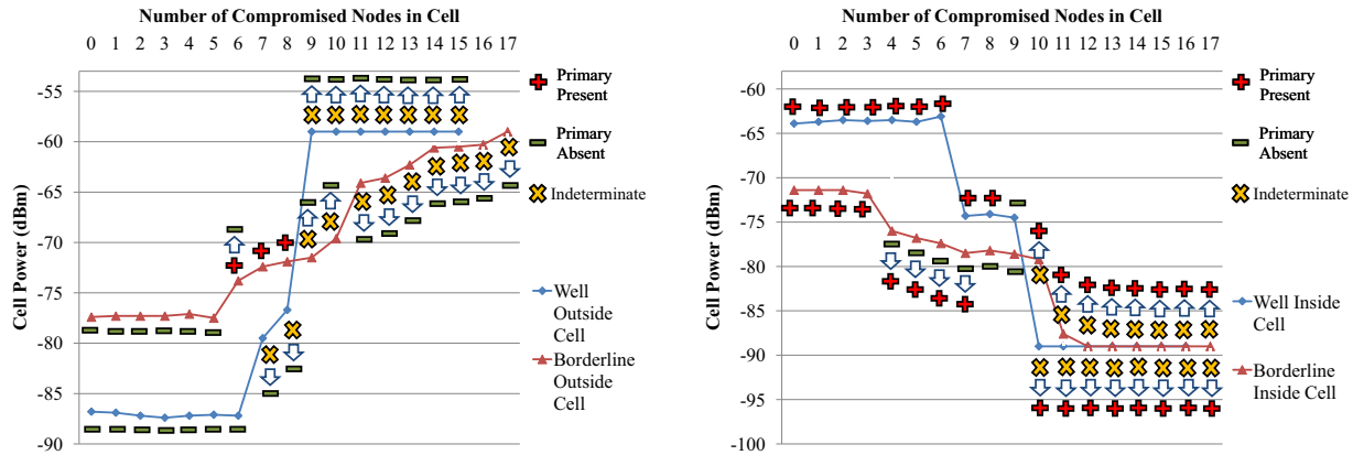
Fig. 5. Exploitation (left) and Vandalism (right) by Naive Attackers. Arrows represent change of final detection outcome based on extensions in Section VI.
